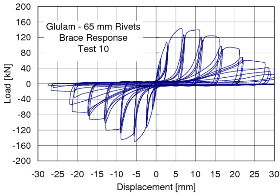
(c) (from Popovski and Karacabeyli 2008)
