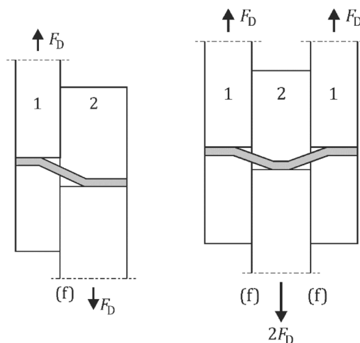
Figure 3: Ductile failure mode with two plastic hinges per shear plane in a fastener.
