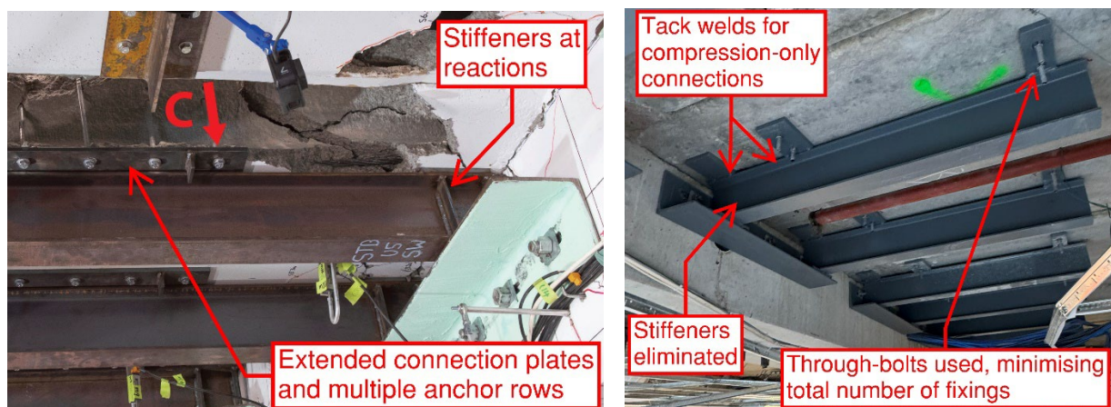
Figure 6: ReCast strongback detailing (left) (Büker et al, 2022), 80TT strongback detailing (right)
